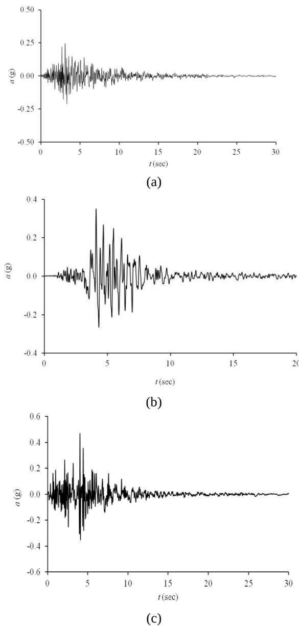
Fig. 3 Input acceleration time history for (a) Loma Prieta earthquake (b) Tolmezzo earthquake and (c) Northridge earthquake
