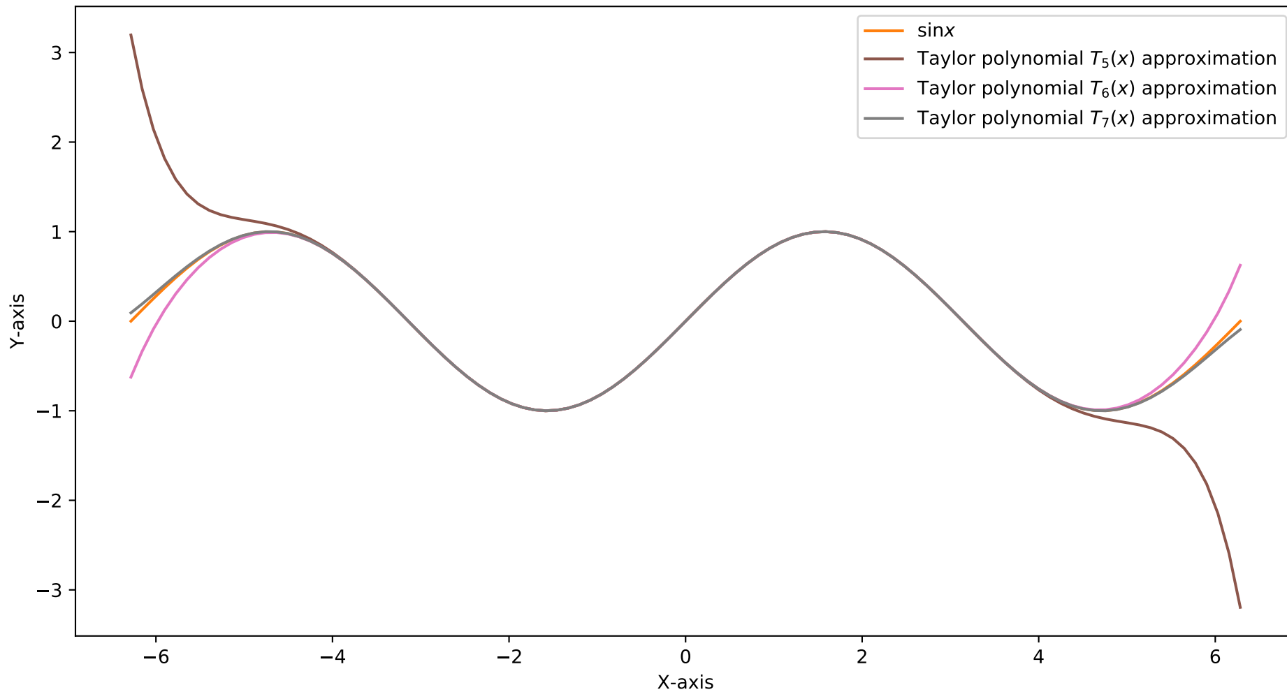
Taylor polynomial T_n(x) approximation of f(x) = \sin x = x - x^3/3! + x^5/5! - \dots
