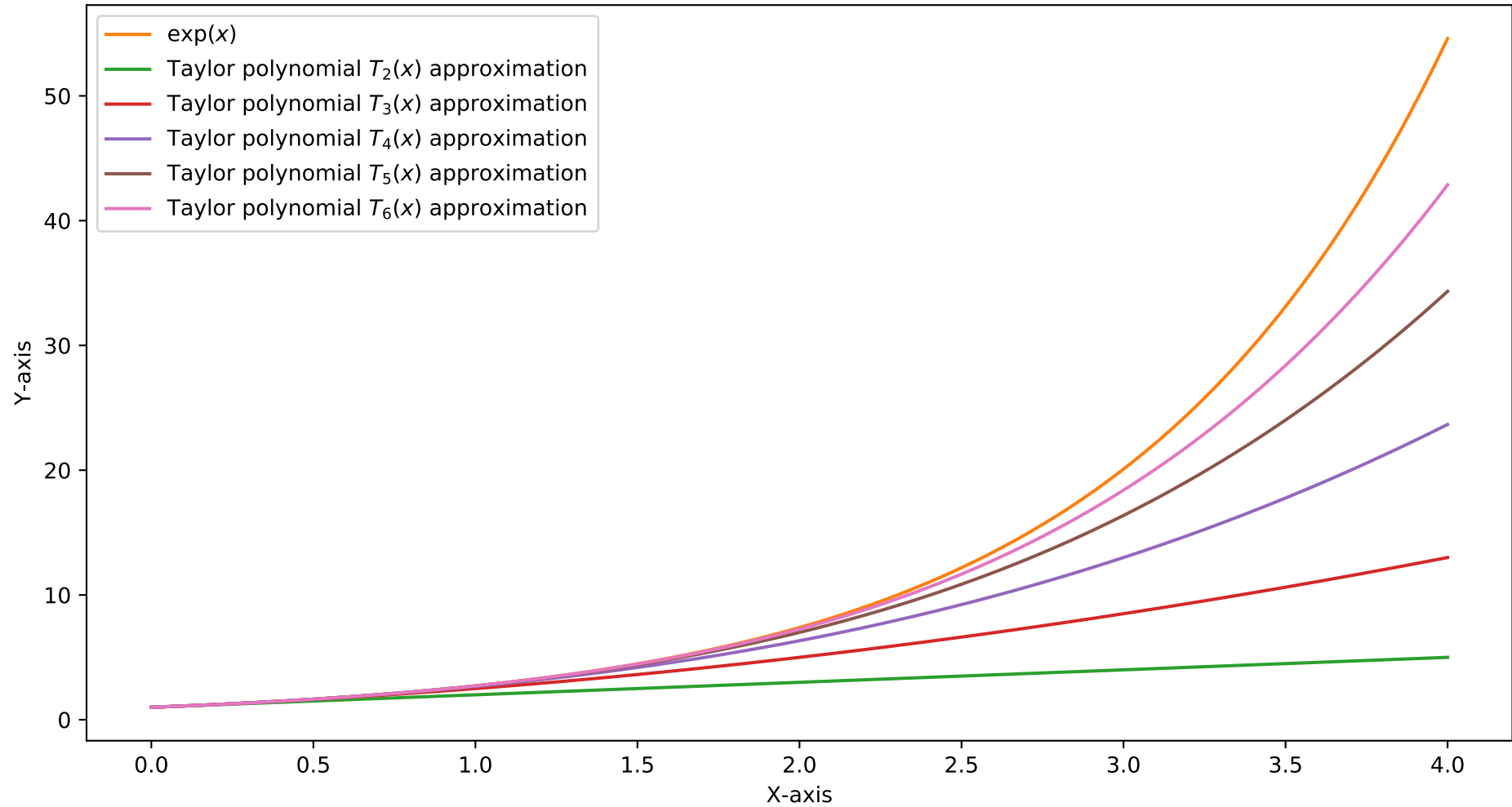
Taylor polynomial T_n(x) approximation of f(x) = \exp(x) = 1 + x + x^2/2! + x^3/3! + \dots
