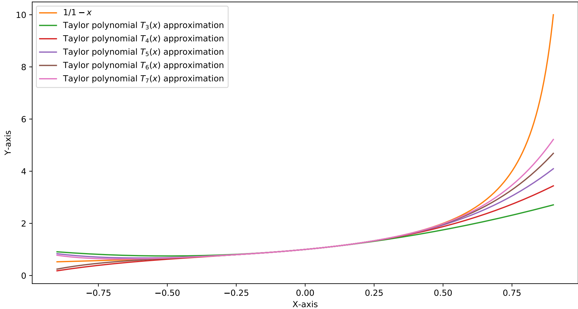
Taylor polynomial T_n(x) approximation of f(x) = 1/1 - x = 1 + x + x^2 + x^3 + \dots
