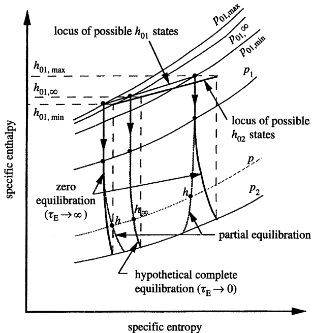
Figure 4. Variation of state for a fluid particle passing through a blade row.
