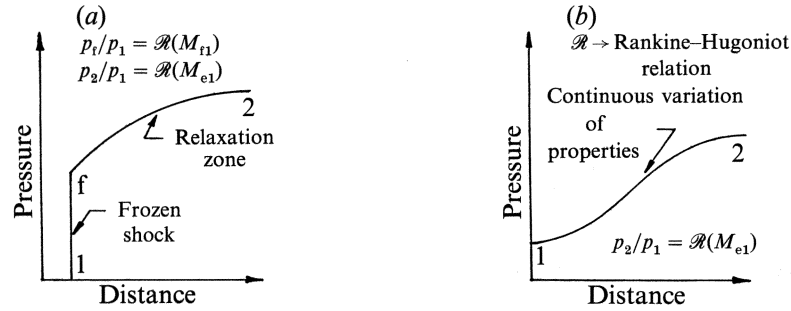
FIGURE 2. Schematic structure of shock waves in a relaxing medium. (a) Partly dispersed shock wave, M_{e1} > 1 , M_{f1} > 1 . (b) Fully dispersed shock wave, M_{e1} > 1 , M_{f1} \leq 1 .
