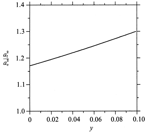
FIGURE 3. Variation of a_r^2/a_e^2 with wetness fraction; p = 0.35 bar.
