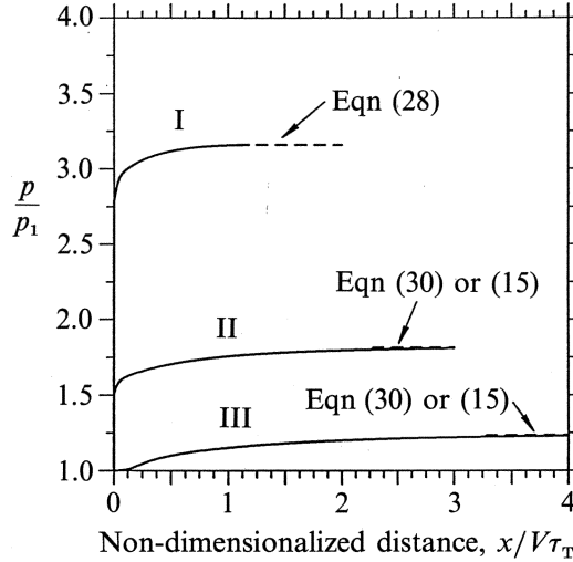
FIGURE 13. Comparison of asymptotic pressure profiles with generalized Rankine-Hugoniot equations: I, partly dispersed with complete evaporation ( p_1 = 0.35 bar, M_{t1} = 1.6 , y_1 = 0.05 , r_1 = 0.1 \mu\text{m} ); II, equilibrium partly dispersed ( p_1 = 0.35 bar, M_{t1} = 1.2 , y_1 = 0.05 , r_1 = 0.1 \mu\text{m} ); III, equilibrium fully dispersed ( p_1 = 0.35 bar, M_{t1} = 0.97 , y_1 = 0.1 , r_1 = 0.1 \mu\text{m} ).
