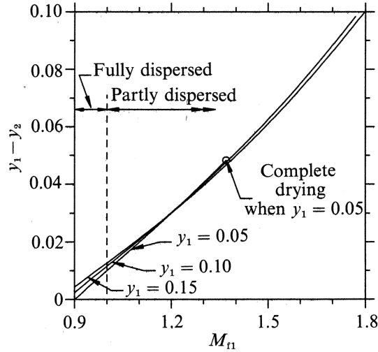
FIGURE 9. Variation of net evaporation with M_{f1} for shock waves in low-pressure steam.
